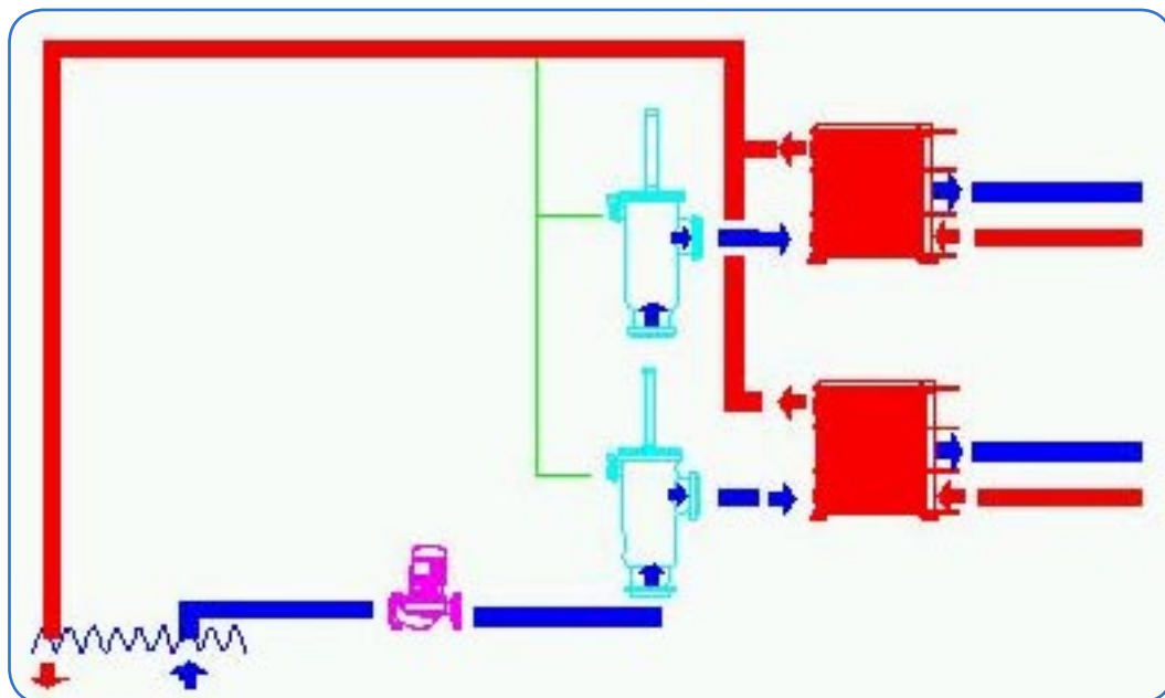
Schematic installation of two Bernoulli Filters protecting two PHEs from clogging.
